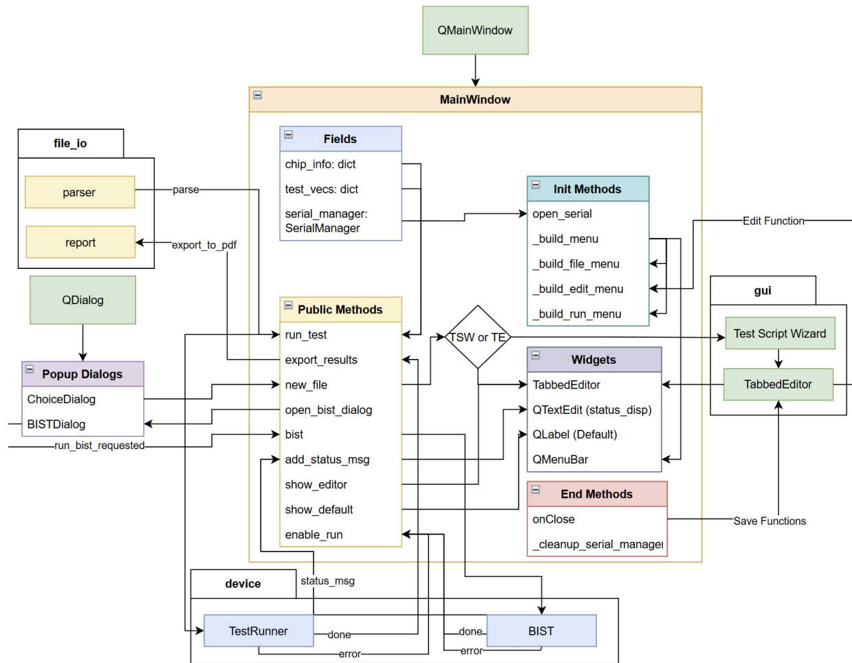
Figure 9. High level overview of the application and the connections to MainWindow
