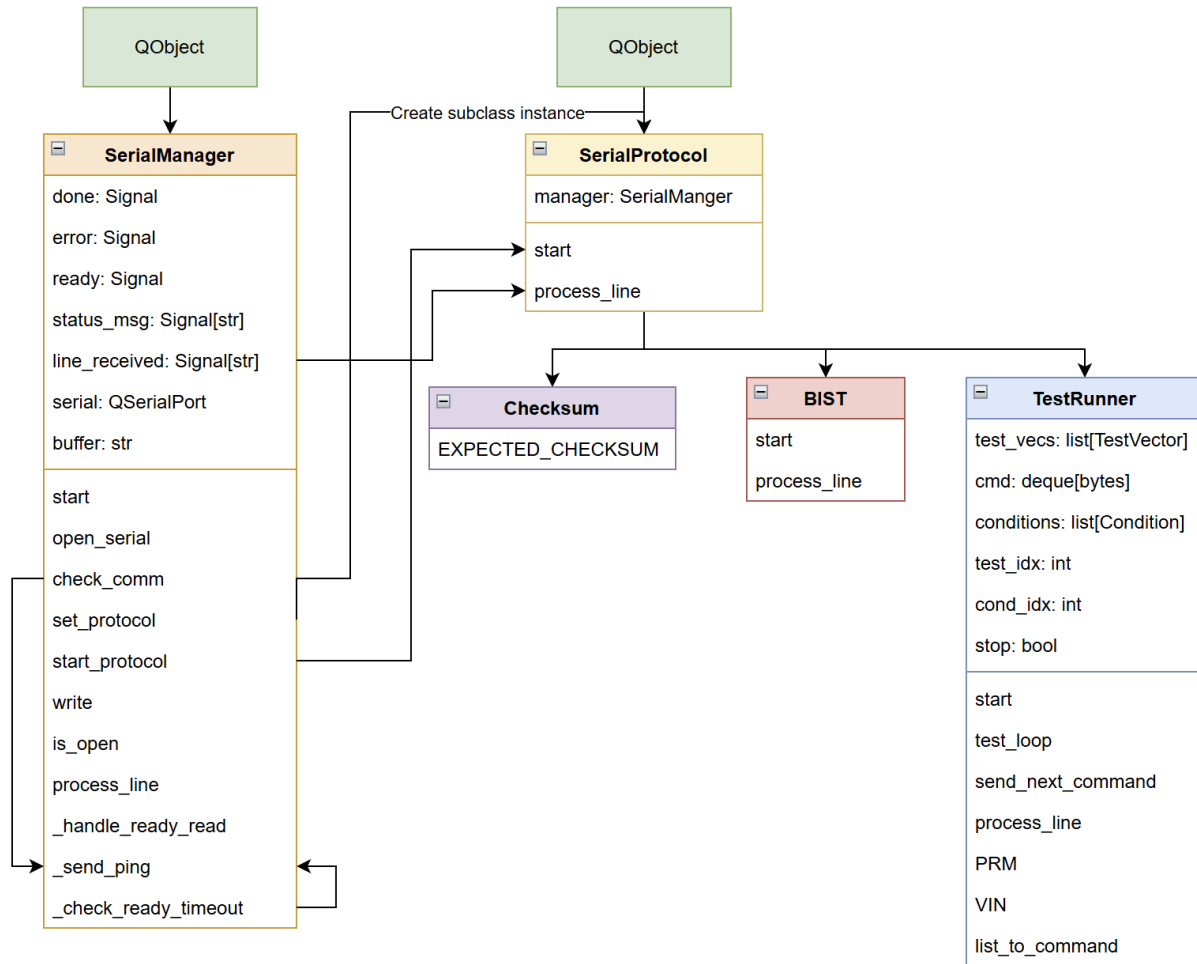
Figure 8: Basic layout of serial_manager.py
