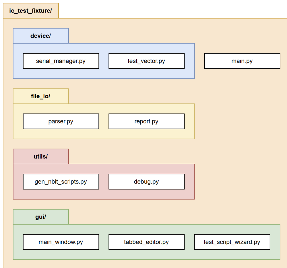
Figure 2. Python project layout
